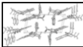
Fig. 2. A packing diagram for the title compound.
