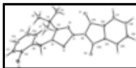
Fig. 1. The molecular structure of the title compound, showing the atom-labelling scheme and 50% probability displacement ellipsoid (arbitrary spheres for H atoms).
